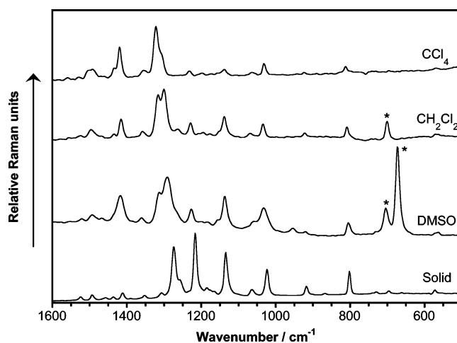
Figure 4. FT-Raman spectra of Me 2 N-T 2 -NO 2 recorded in CCl 4 , CH 2 Cl 2 , and DMSO solutions and in solid state over probe energies of 1600–500 cm -1 . Asterisks denote solvent bands.
