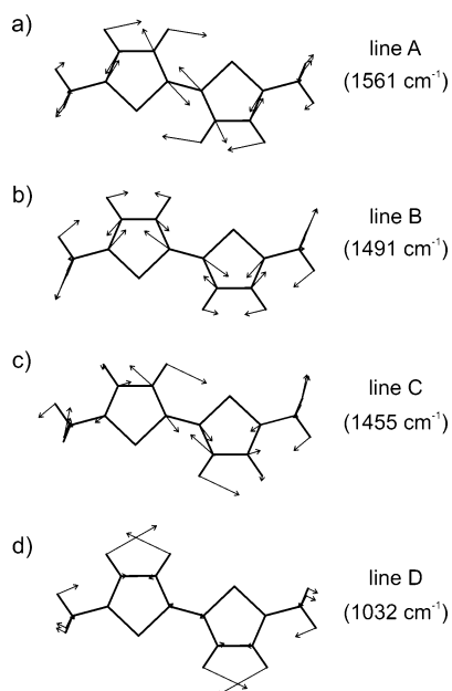
Figure 5. Schematic eigenvectors calculated at the B3LYP/6-31G** level for the most intense Raman-active symmetric vibrations of Me-T 2 -Me ( C 2 symmetry). Calculated wavenumbers are given within parentheses.
